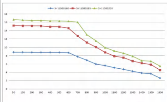
110Series two-phase closed loop stepping motor torque curve
