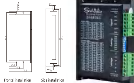
Installation size:
