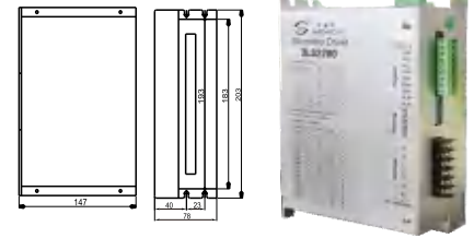
install dimensions
