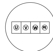
Motor rear cover wiring diagram
