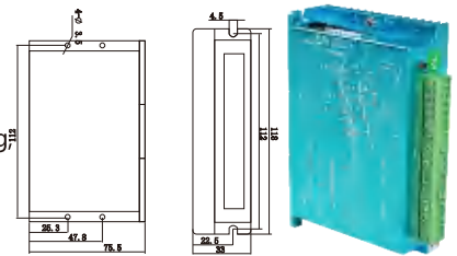
install dimensions
