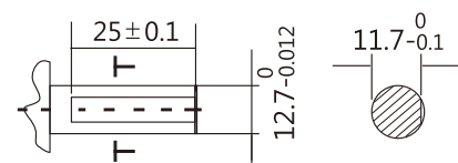
86A4 shaft size
