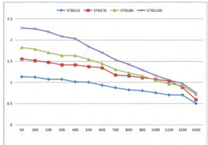
57 Series two-phase stepping motor torque curve
