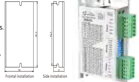
Installation size:
