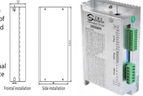
Installation size:
