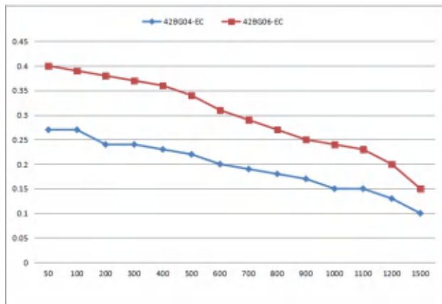
42Series two-phase closed loop stepping motor torque curve
