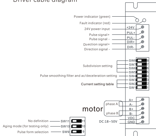
Driver cable diagram
